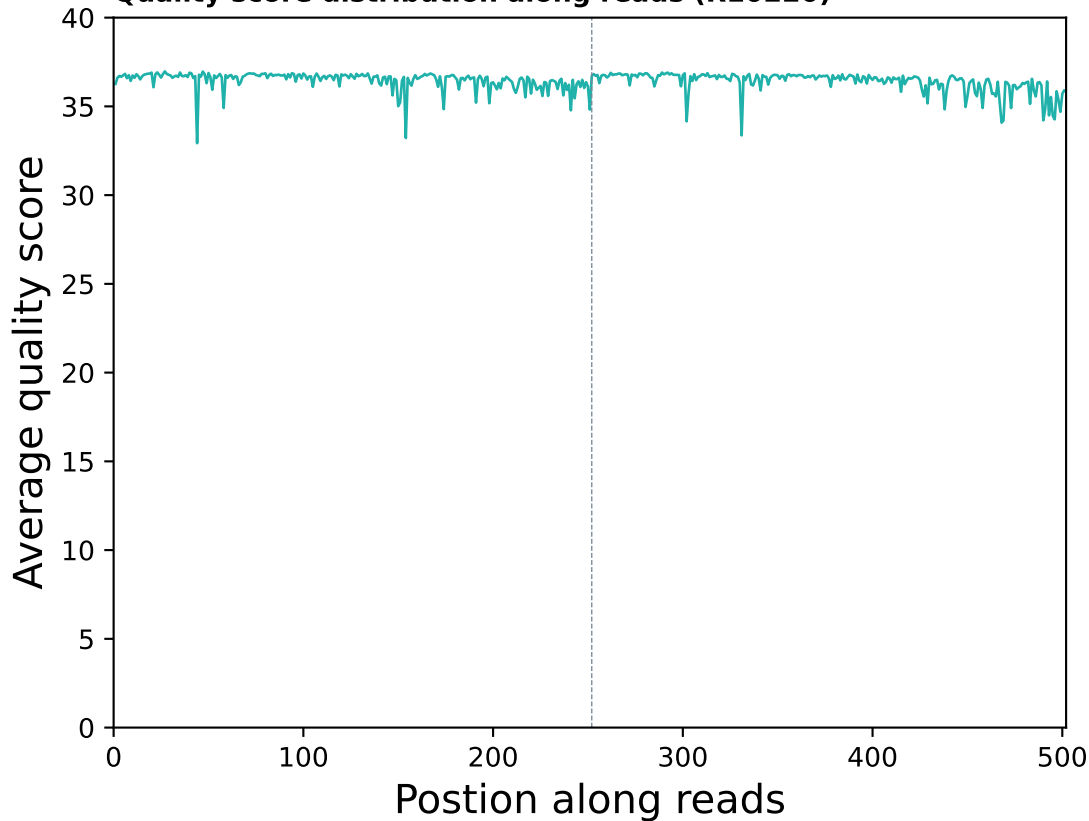
Quality score distribution along reads (R10220)
